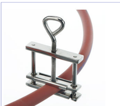
Pinch cock type HOFFMANN, heavy type
